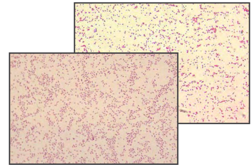
Gram Stain
